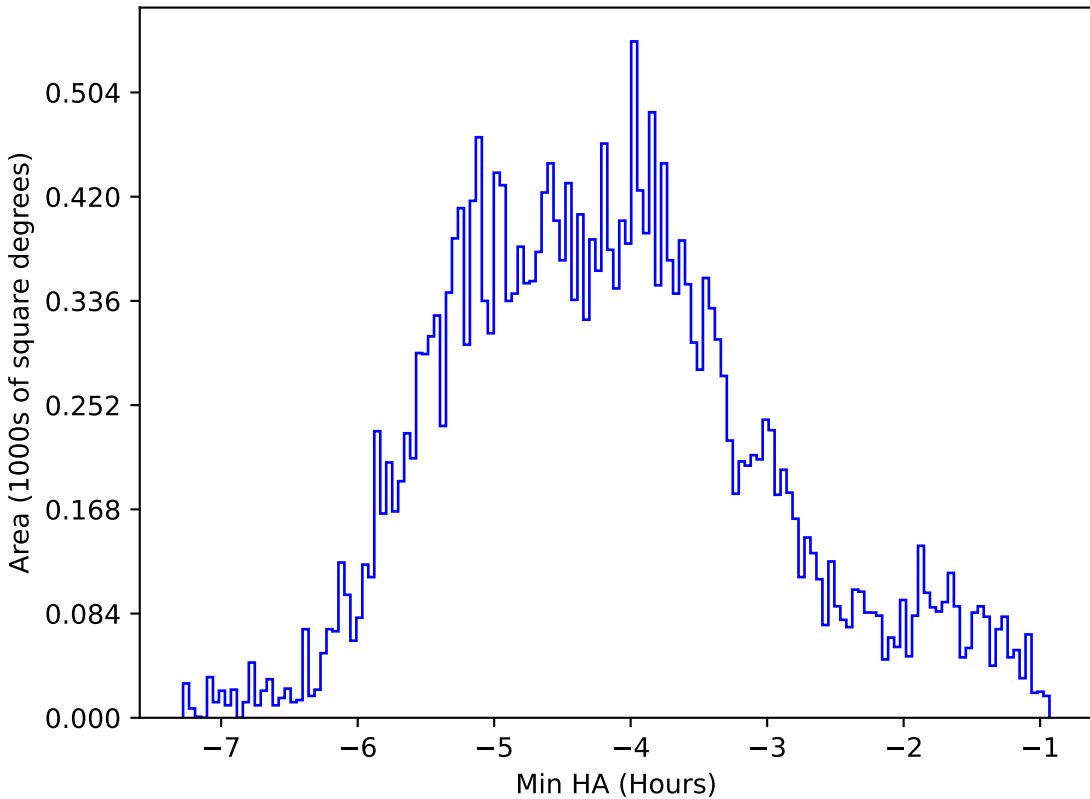
start_date_do-360v3.4_10yrs All sky r band: Min HA
