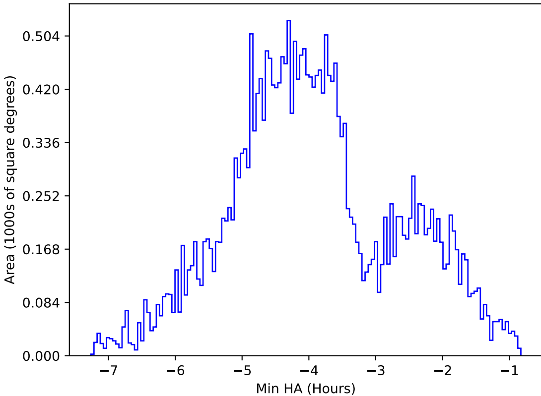
start_date_do-360v3.4_10yrs All sky g band: Min HA
