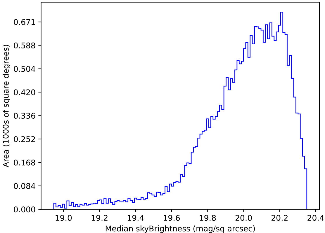
start_date_do-360v3.4_10yrs Yr 1 i band: Median skyBrightness
