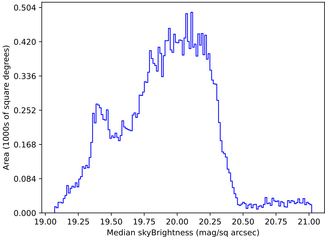
start_date_do-360v3.4_10yrs Yr 1 all bands: Median skyBrightness
