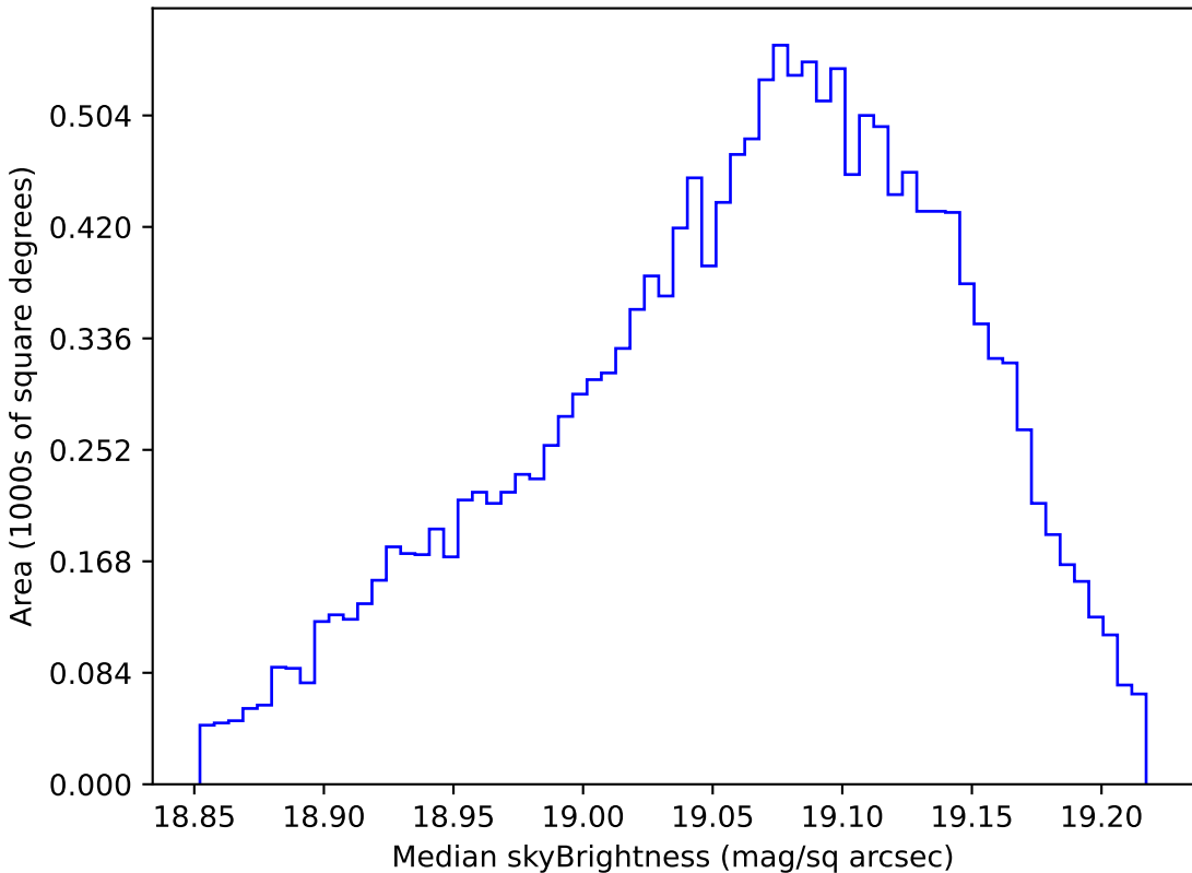
start_date_do-360v3.4_10yrs WFD z band: Median skyBrightness
