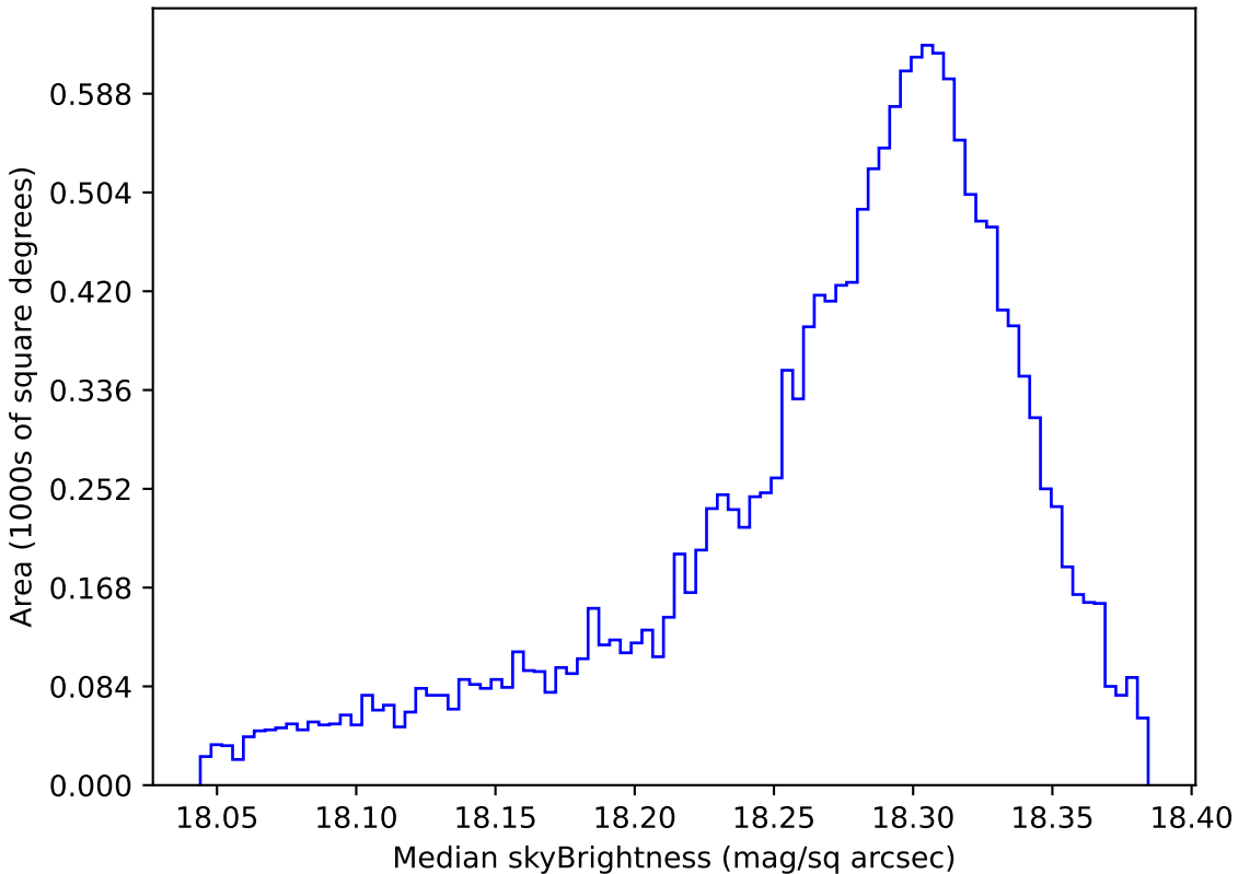
start_date_do-360v3.4_10yrs WFD y band: Median skyBrightness
