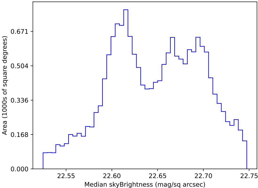
start_date_do-360v3.4_10yrs WFD u band: Median skyBrightness
