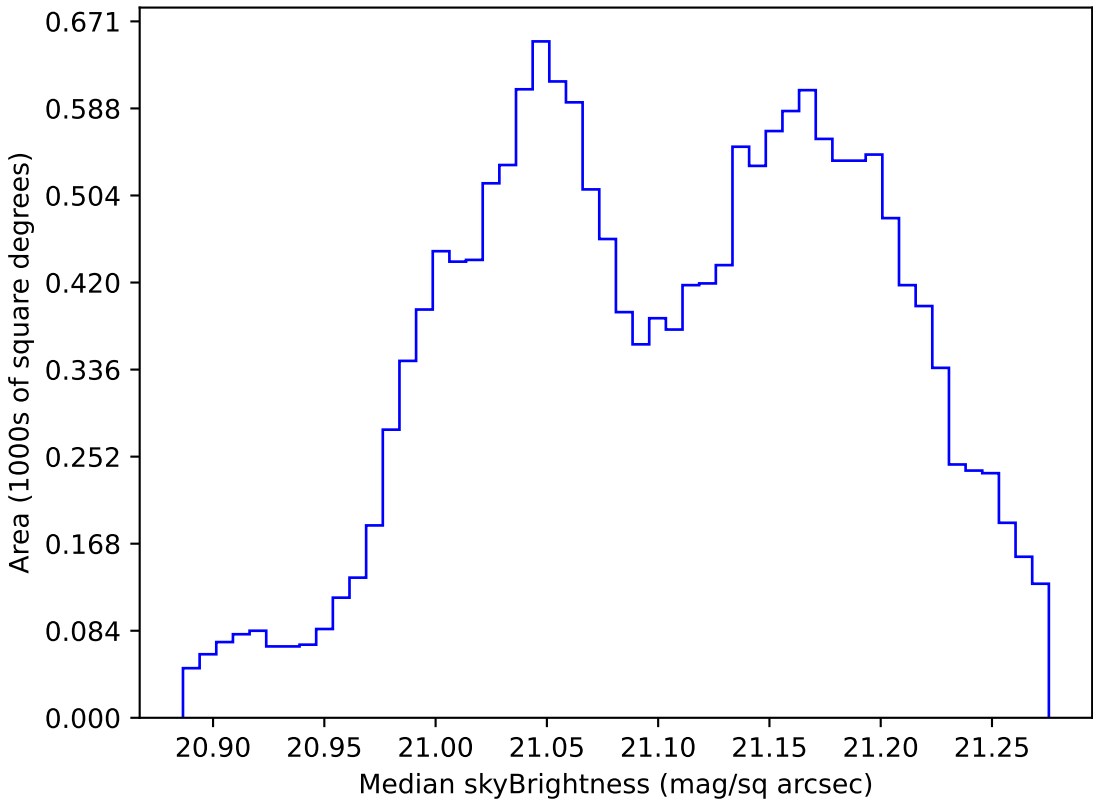
start_date_do-360v3.4_10yrs WFD r band: Median skyBrightness
