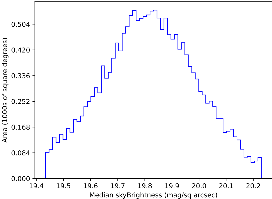
start_date_do-360v3.4_10yrs WFD all bands: Median skyBrightness
