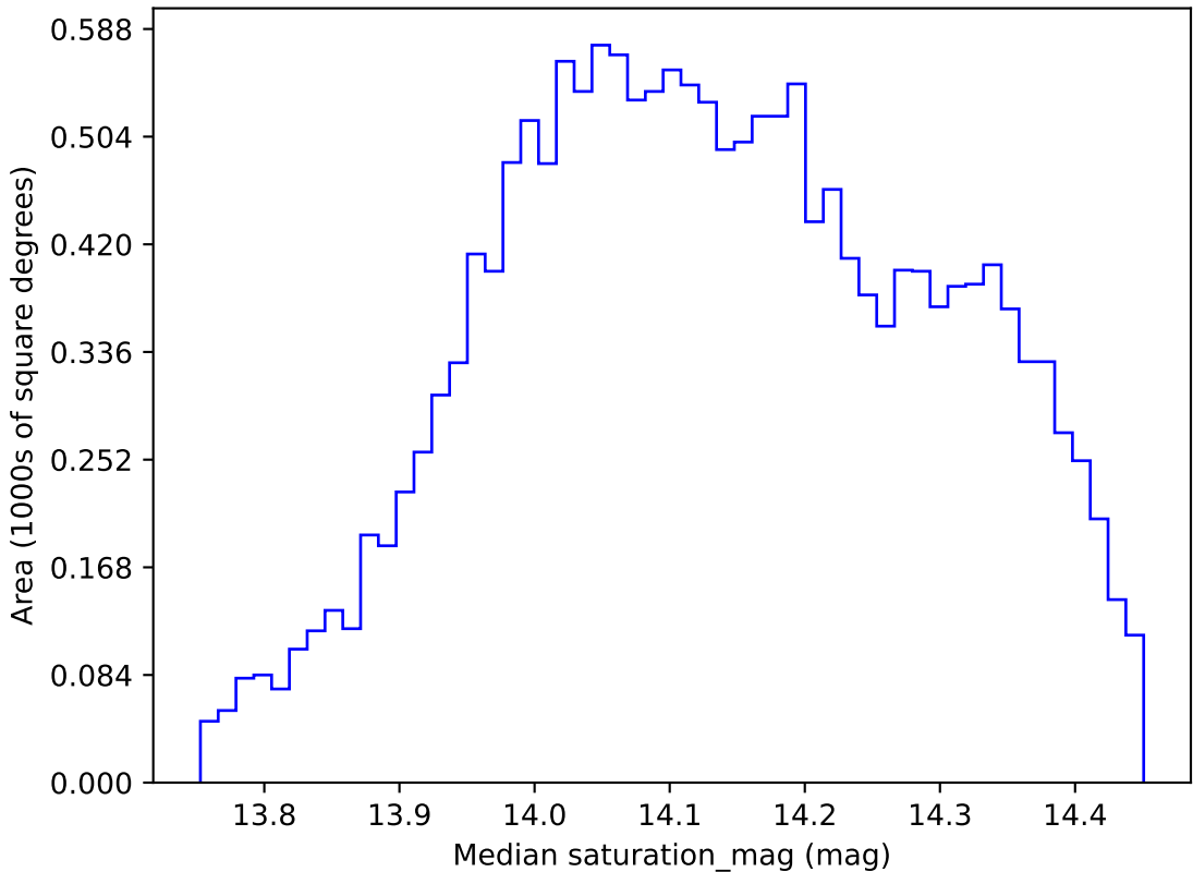
start_date_do-360v3.4_10yrs WFD z band: Median saturation_mag
