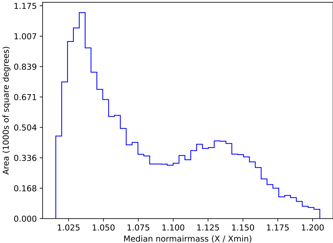
start_date_do-360v3.4_10yrs WFD g band: Median normairmass
