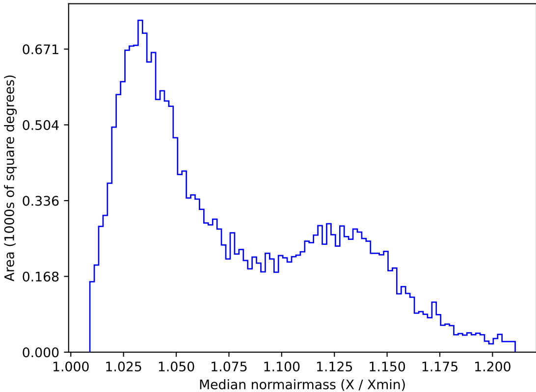
start_date_do-360v3.4_10yrs All sky u band: Median normairmass
