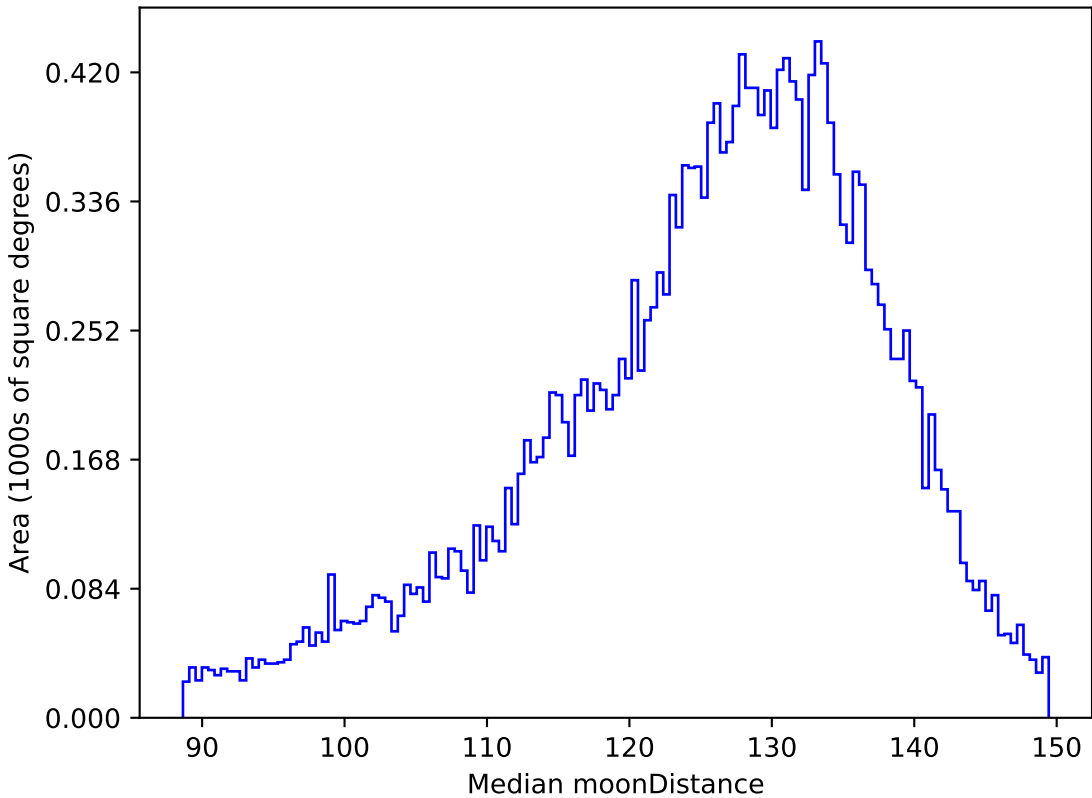
start_date_do-360v3.4_10yrs All sky u band: Median moonDistance
