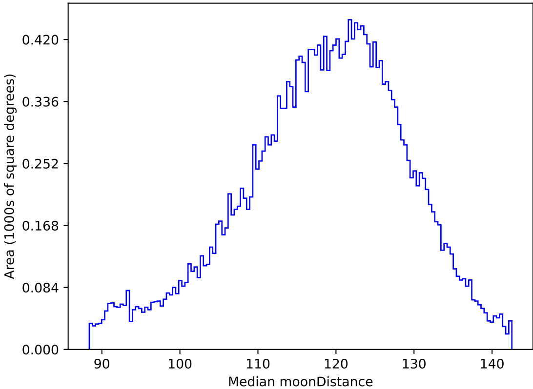
start_date_do-360v3.4_10yrs All sky g band: Median moonDistance
