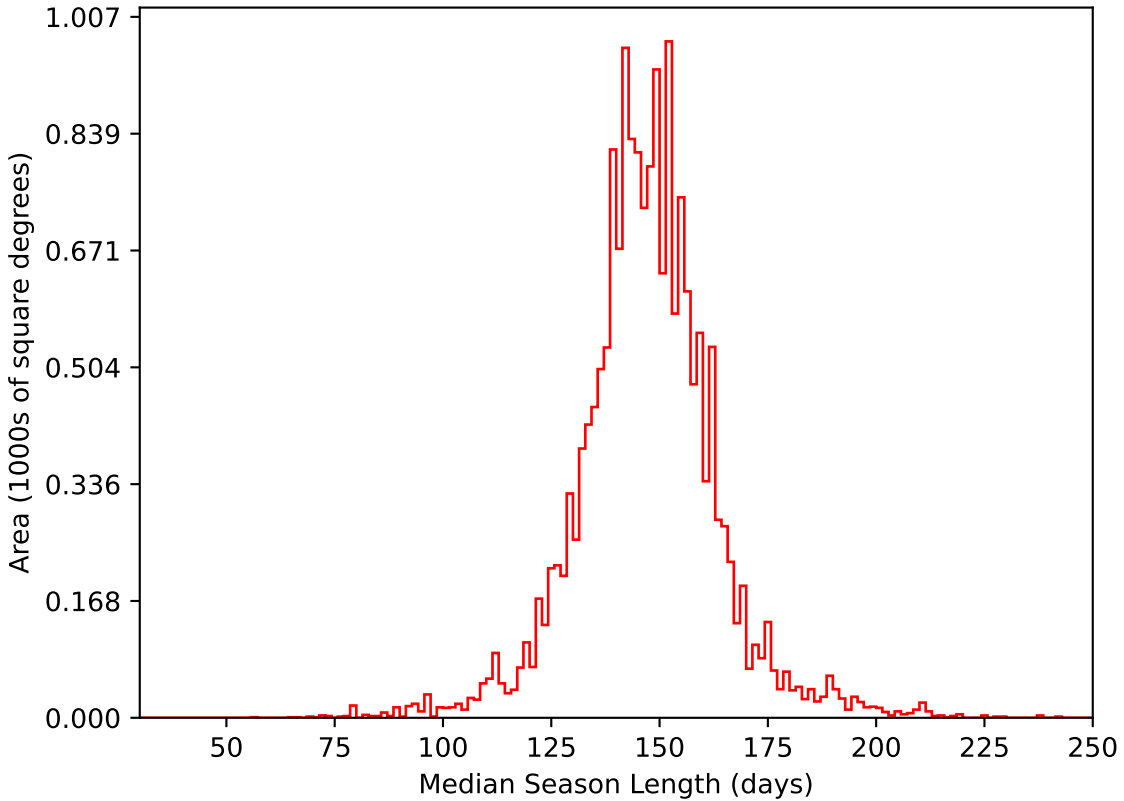
start_date_do-360v3.4_10yrs WFD i band: Median Season Length
