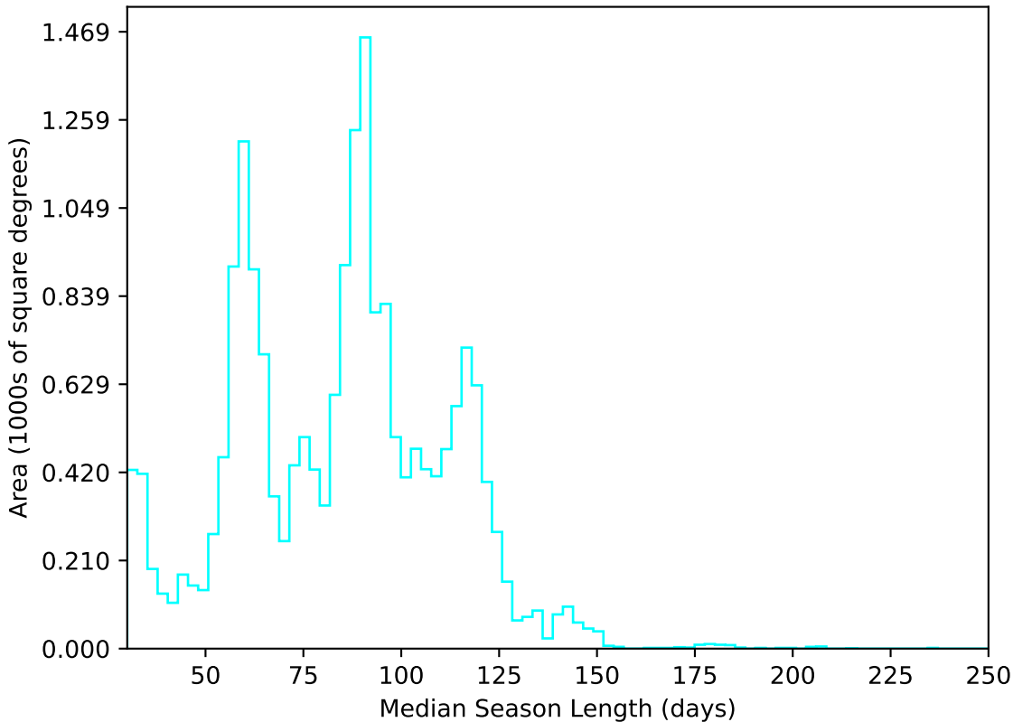
start_date_do-360v3.4_10yrs All sky u band: Median Season Length
