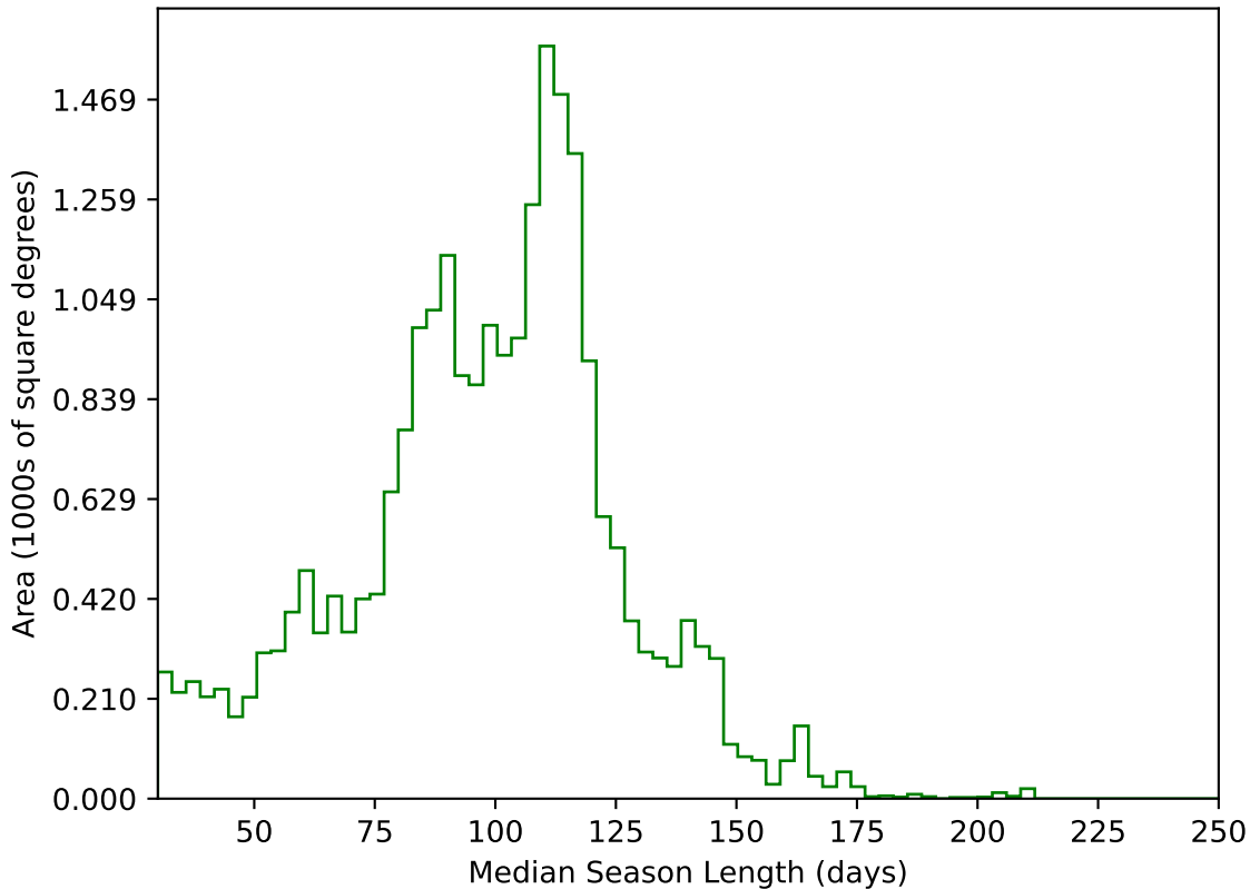
start_date_do-360v3.4_10yrs All sky g band: Median Season Length
