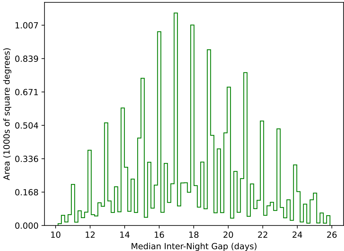
start_date_do-360v3.4_10yrs WFD g band: Median Inter-Night Gap
