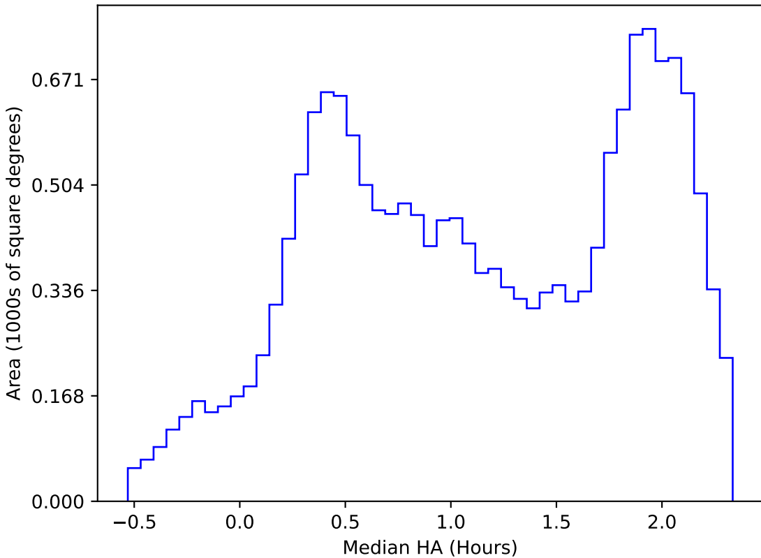
start_date_do-360v3.4_10yrs WFD z band: Median HA
