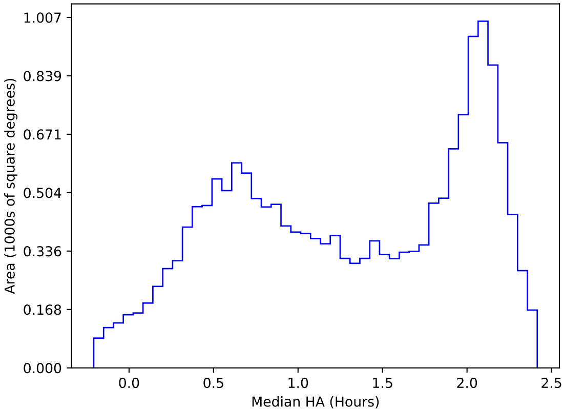
start_date_do-360v3.4_10yrs WFD y band: Median HA
