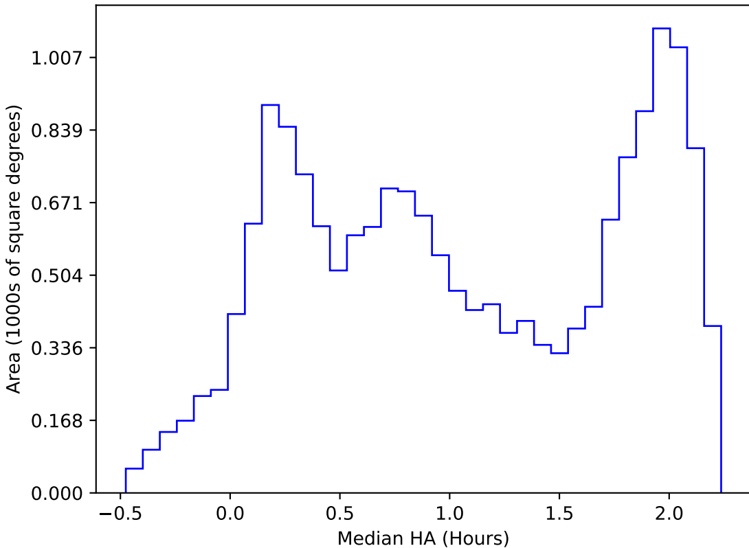
start_date_do-360v3.4_10yrs WFD i band: Median HA
