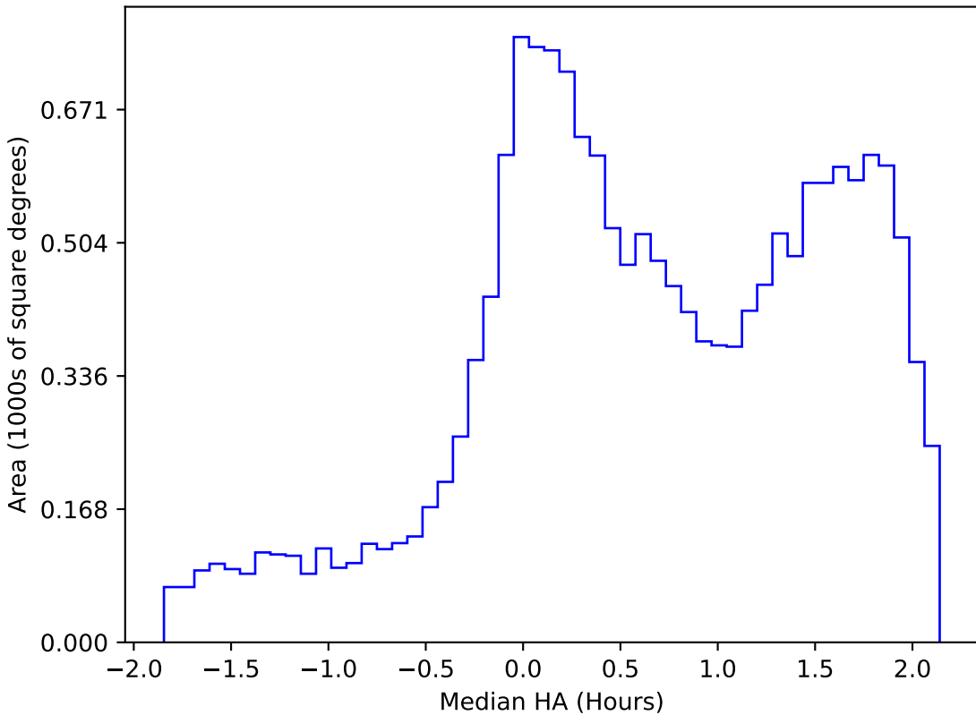
start_date_do-360v3.4_10yrs WFD g band: Median HA
