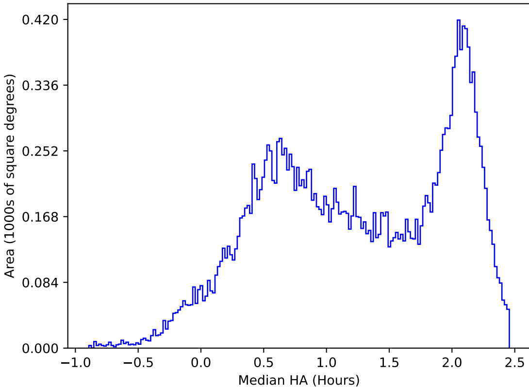
start_date_do-360v3.4_10yrs All sky y band: Median HA
