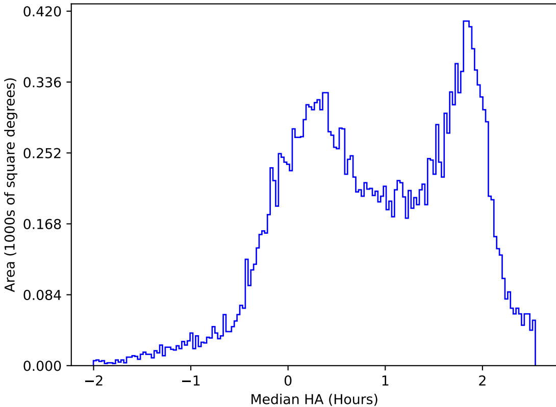
start_date_do-360v3.4_10yrs All sky u band: Median HA
