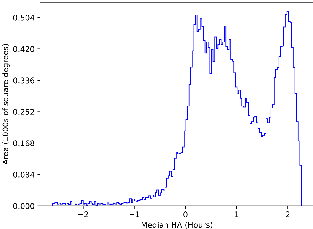
start_date_do-360v3.4_10yrs All sky i band: Median HA
