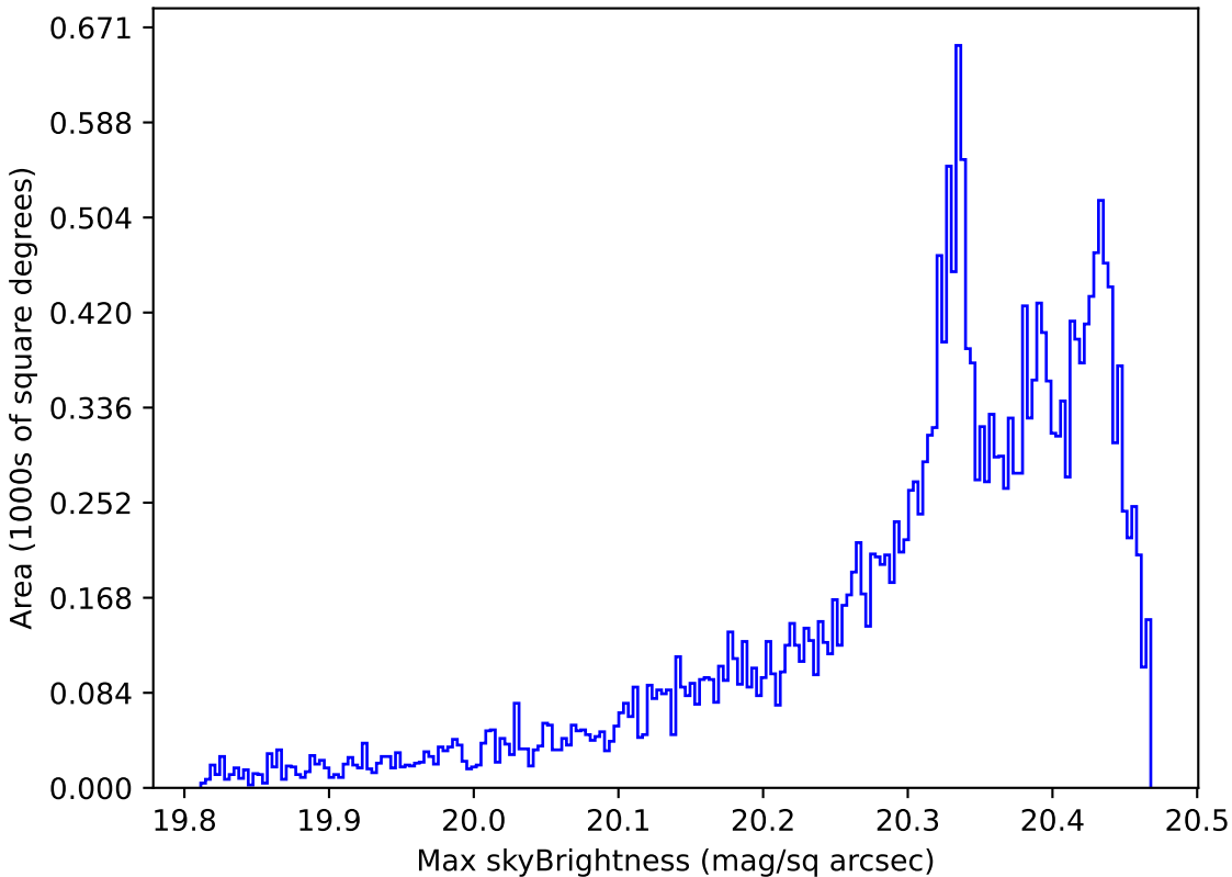
start_date_do-360v3.4_10yrs All sky i band: Max skyBrightness
