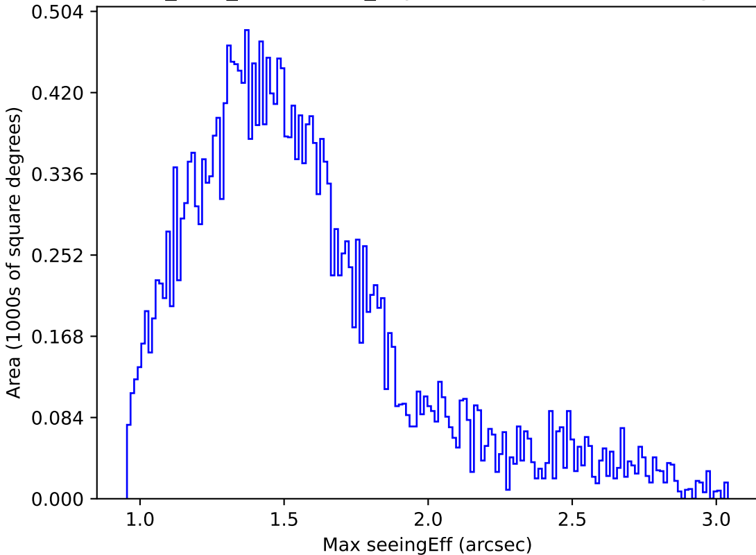
start_date_do-360v3.4_10yrs Yr 1 z band: Max seeingEff
