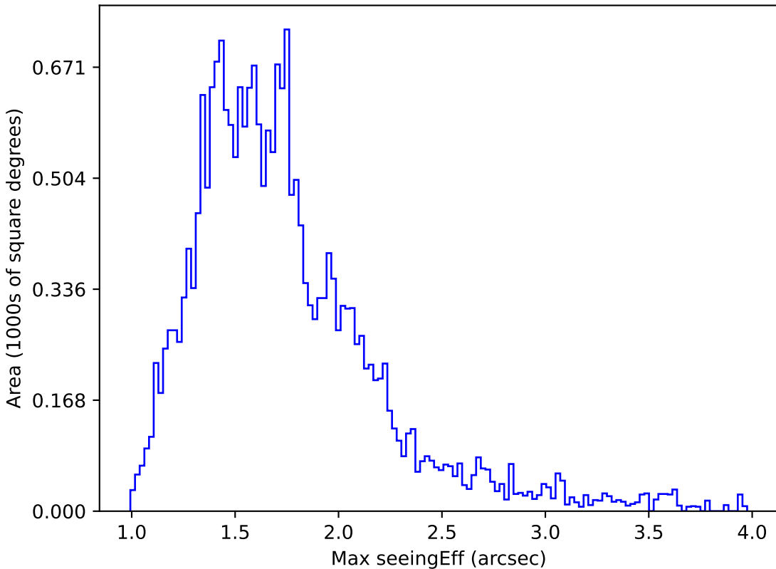
start_date_do-360v3.4_10yrs Yr 1 u band: Max seeingEff
