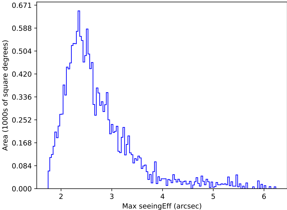
start_date_do-360v3.4_10yrs WFD i band: Max seeingEff
