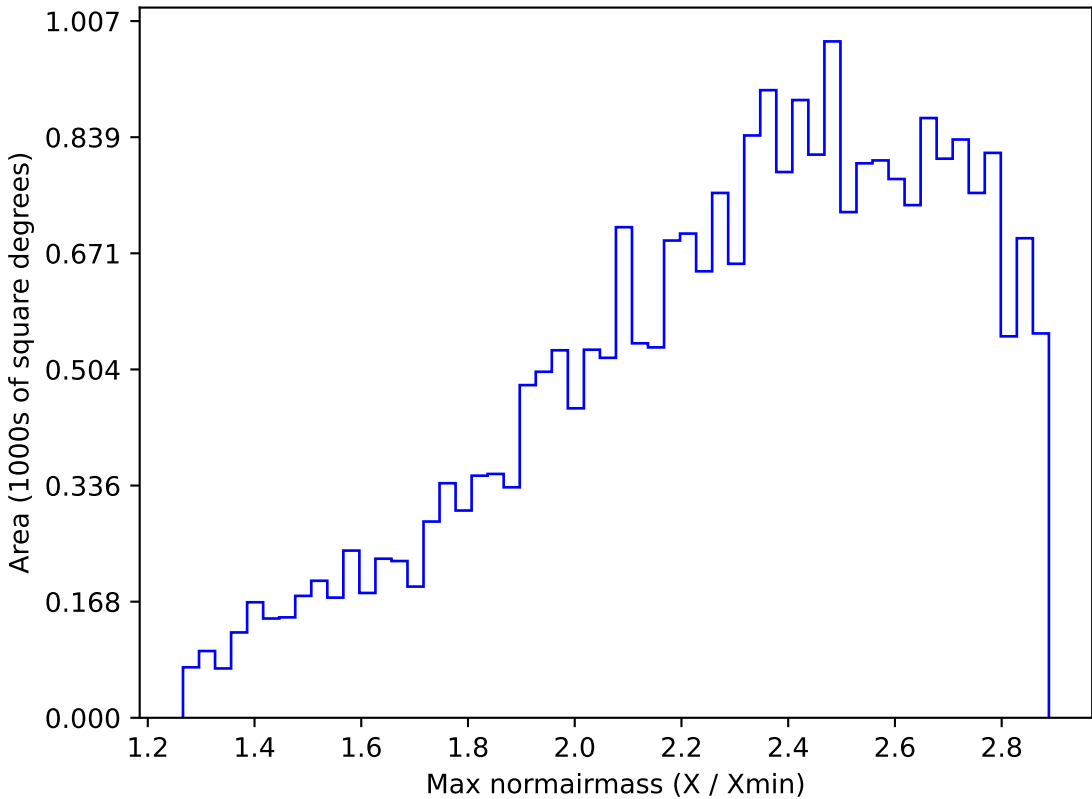
start_date_do-360v3.4_10yrs All sky all bands: Max normairmass
