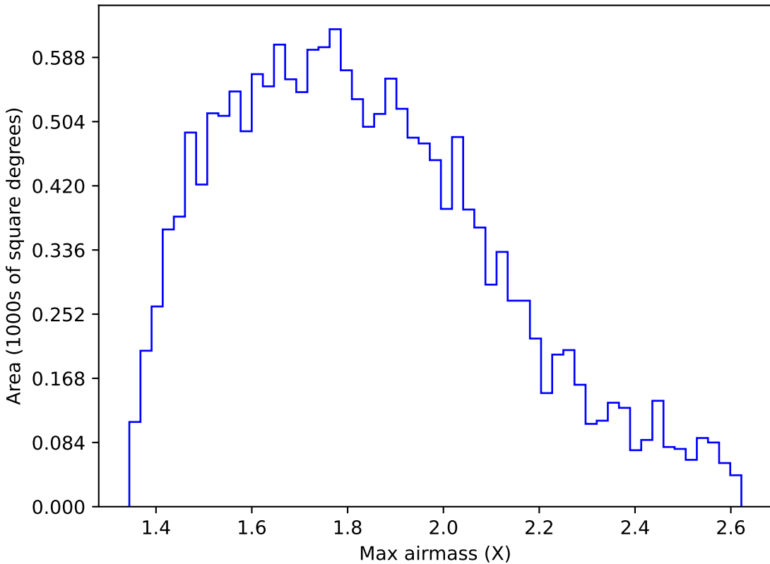
start_date_do-360v3.4_10yrs WFD u band: Max airmass
