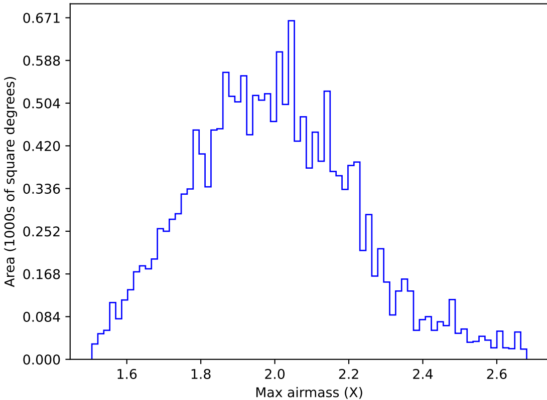
start_date_do-360v3.4_10yrs WFD g band: Max airmass
