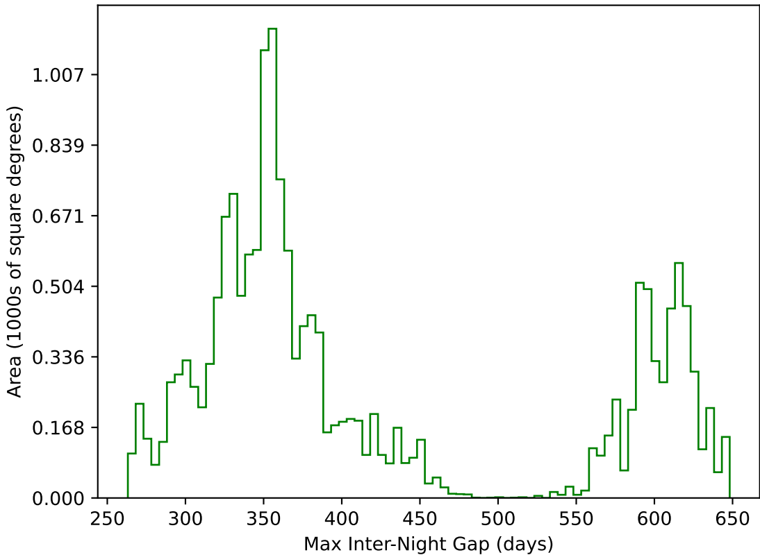
start_date_do-360v3.4_10yrs WFD g band: Max Inter-Night Gap
