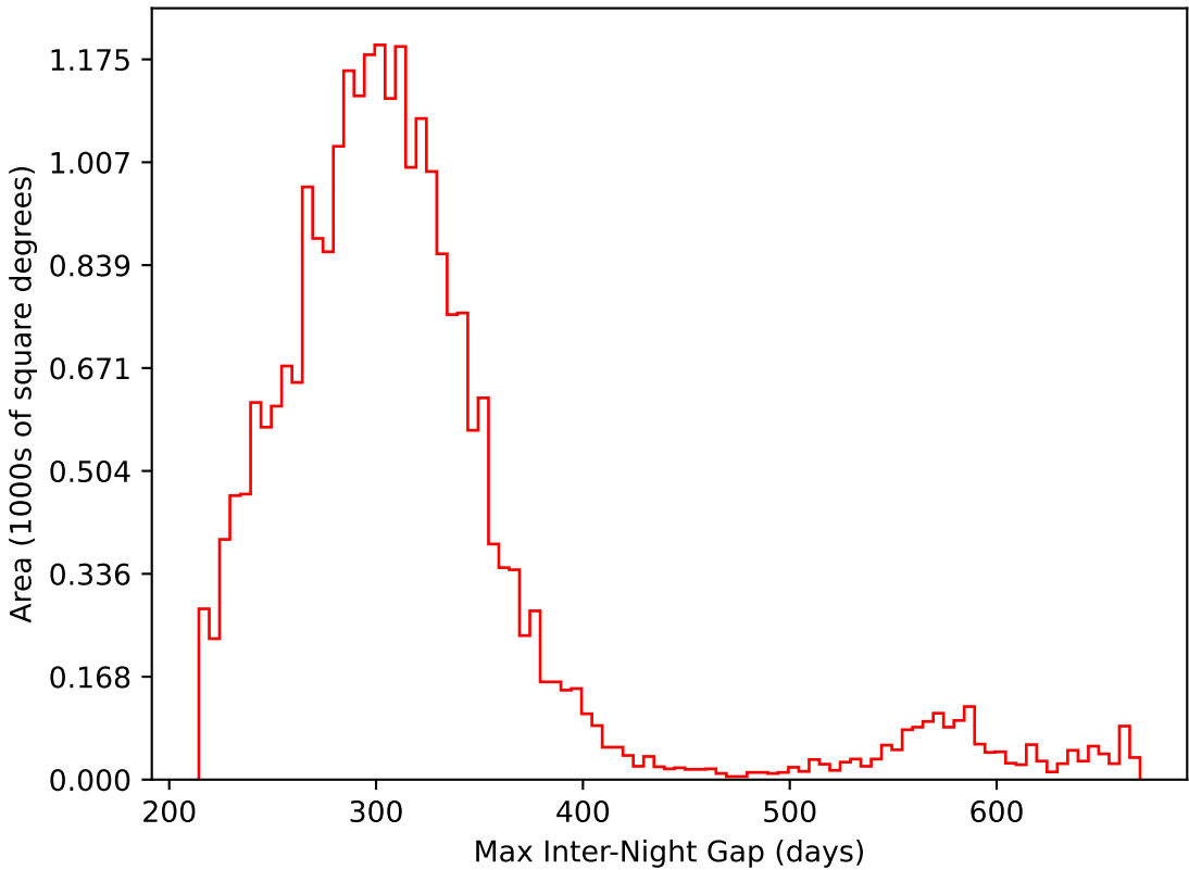
start_date_do-360v3.4_10yrs All sky i band: Max Inter-Night Gap
