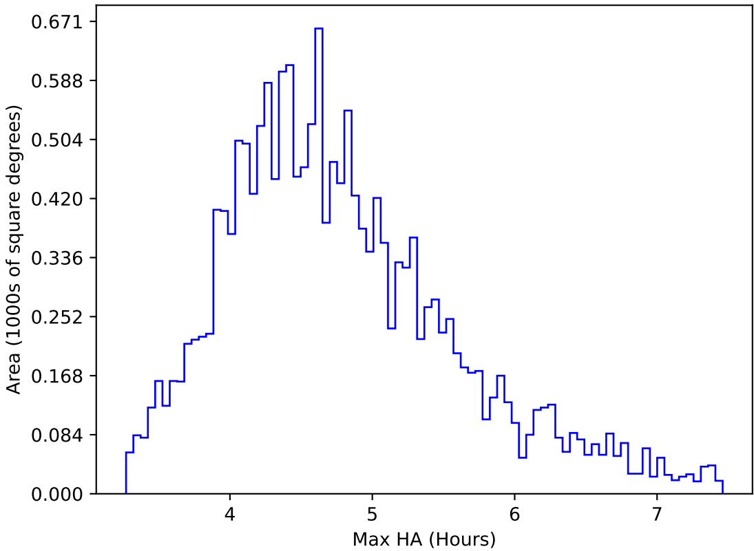
start_date_do-360v3.4_10yrs WFD y band: Max HA
