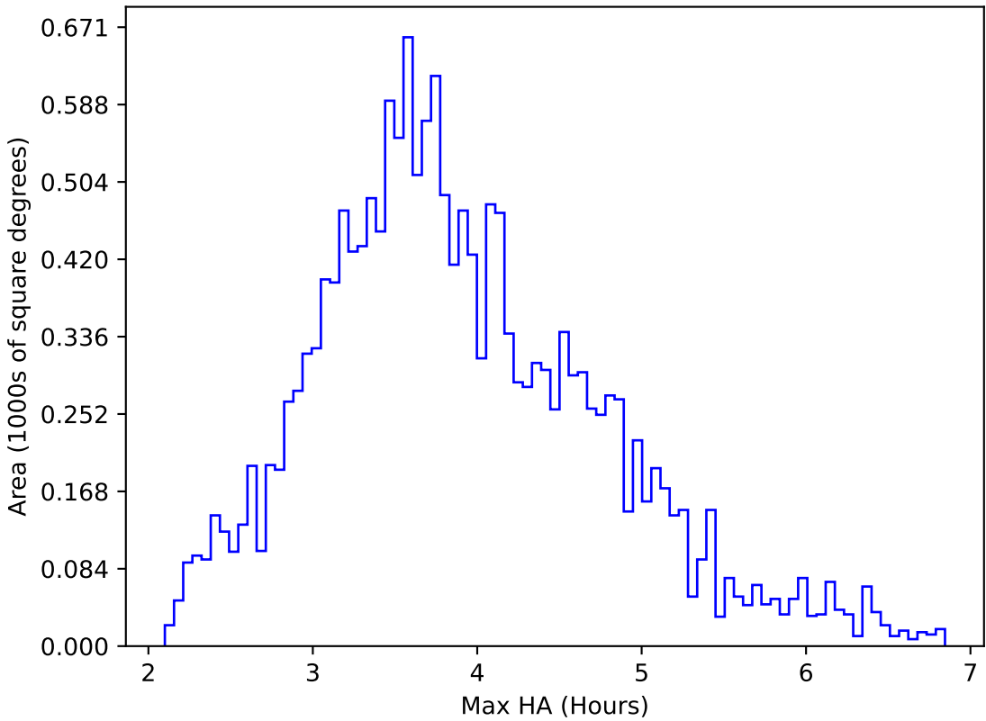
start_date_do-360v3.4_10yrs WFD u band: Max HA
