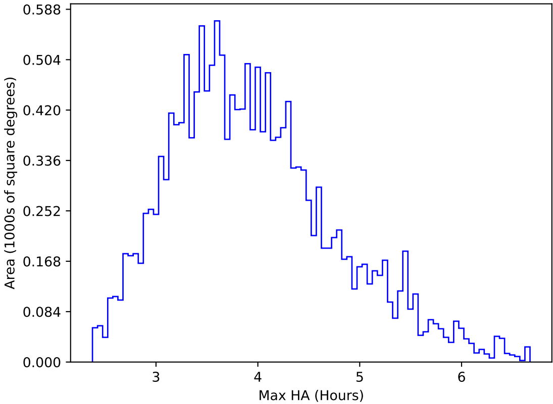
start_date_do-360v3.4_10yrs WFD g band: Max HA
