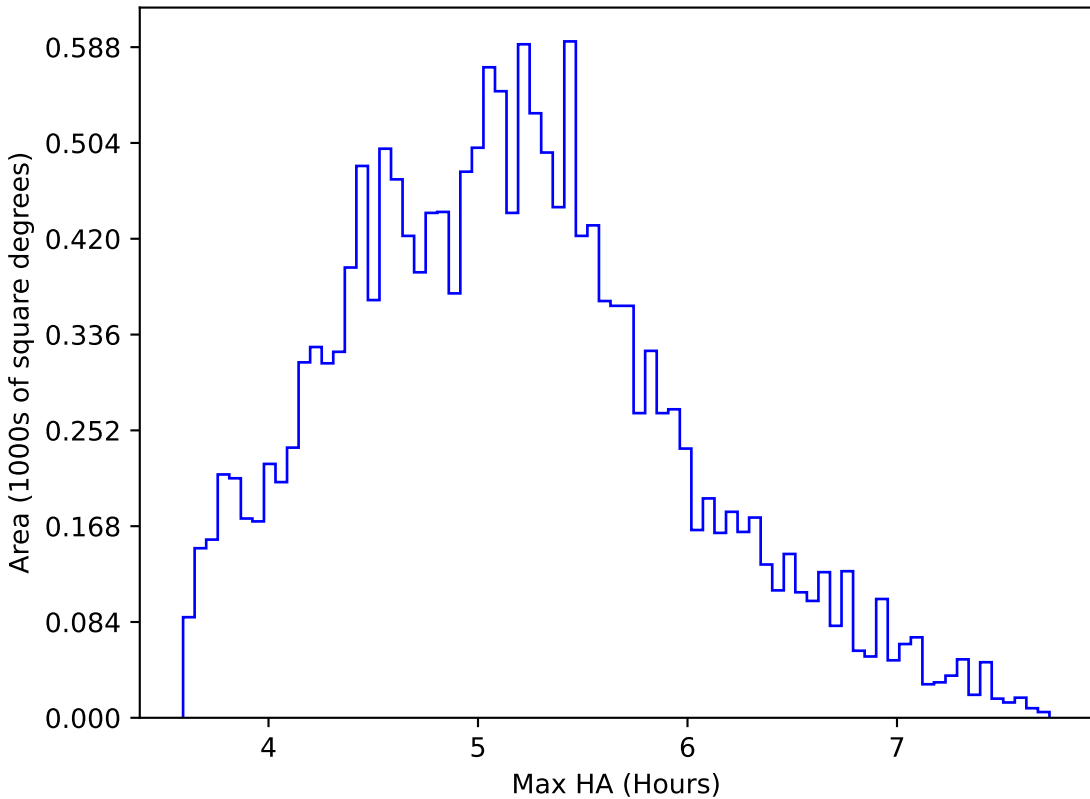
start_date_do-360v3.4_10yrs WFD all bands: Max HA
