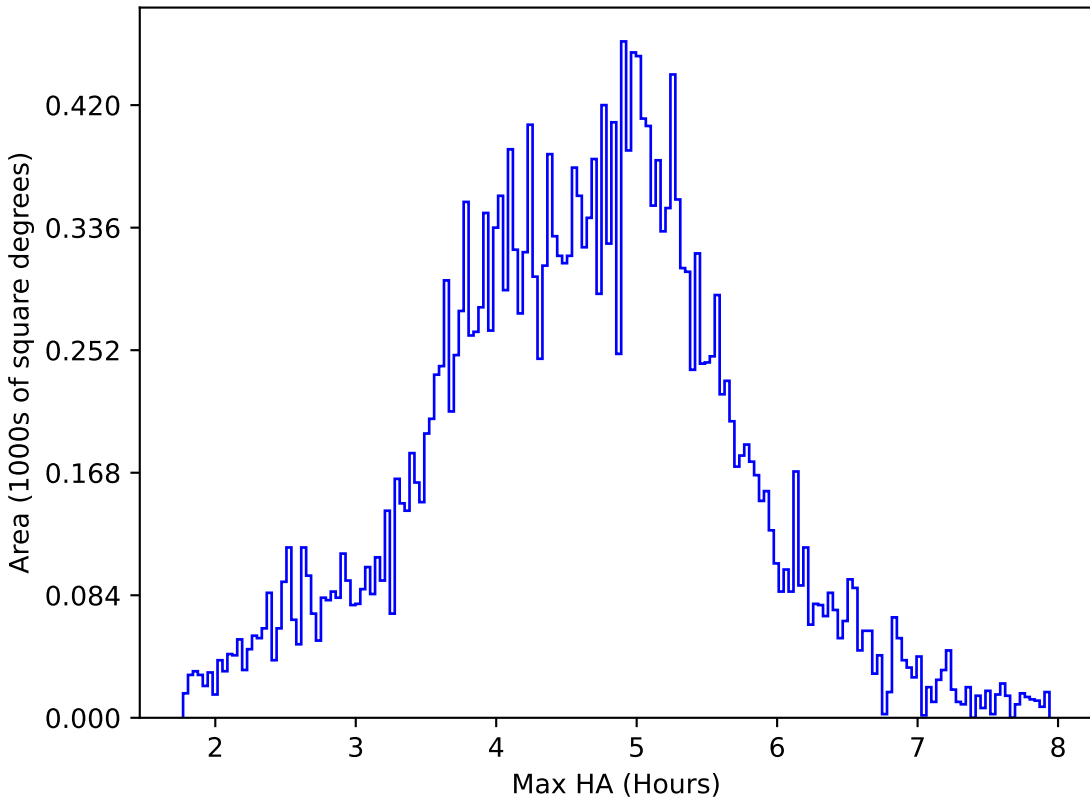
start_date_do-360v3.4_10yrs All sky z band: Max HA
