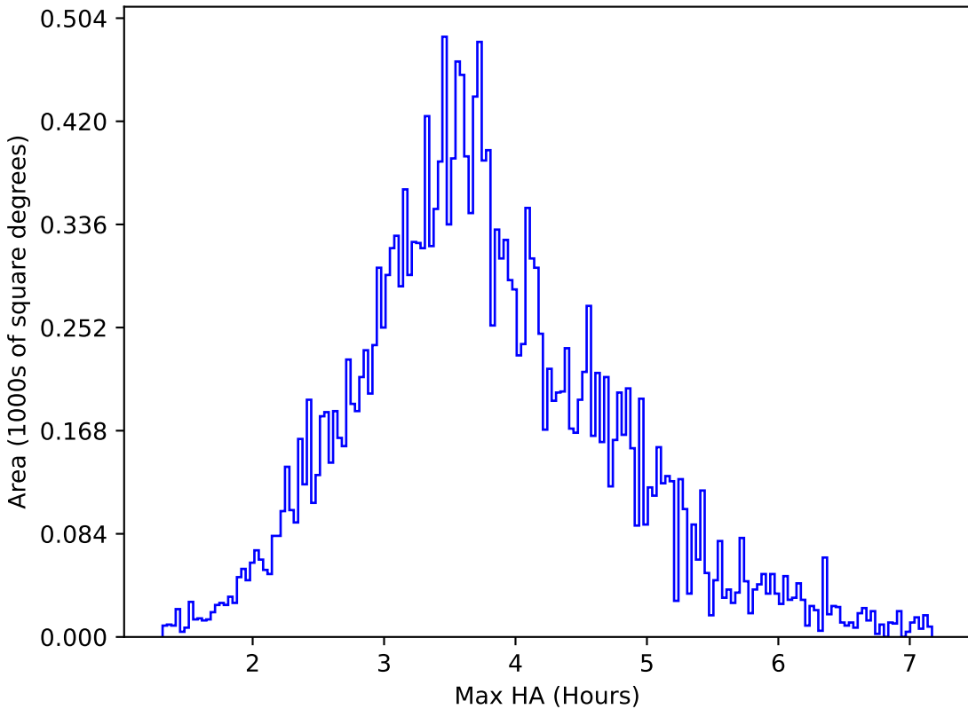
start_date_do-360v3.4_10yrs All sky u band: Max HA
