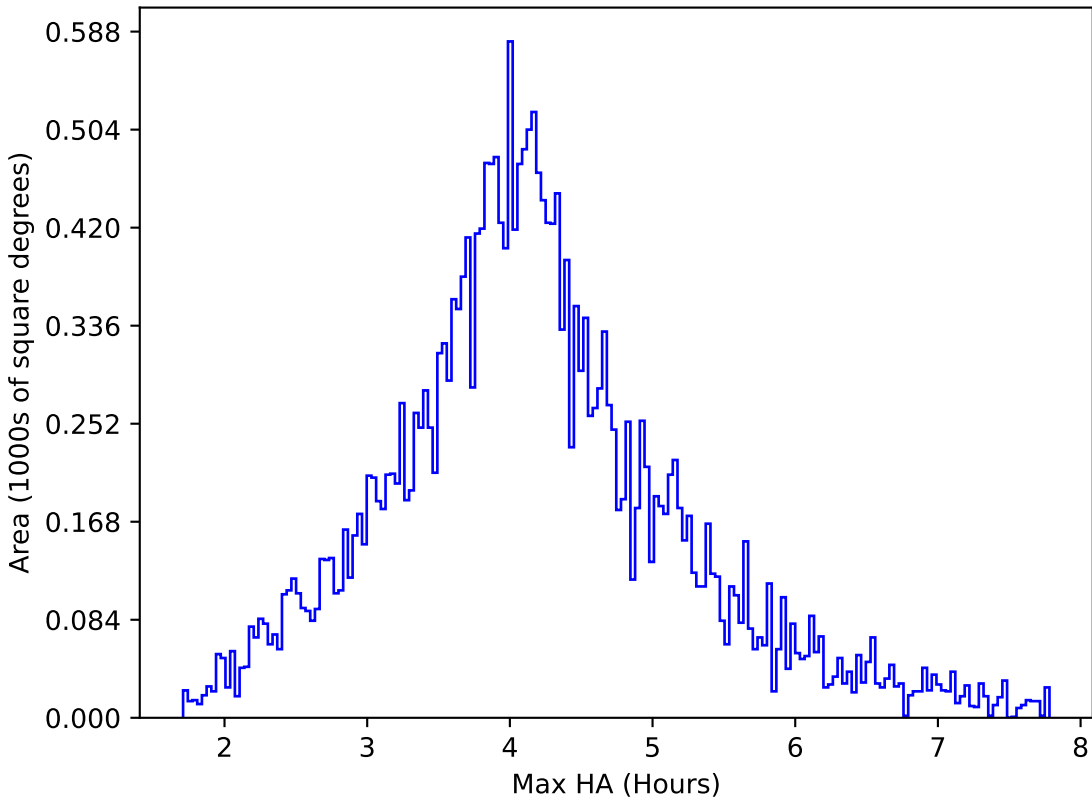
start_date_do-360v3.4_10yrs All sky r band: Max HA
