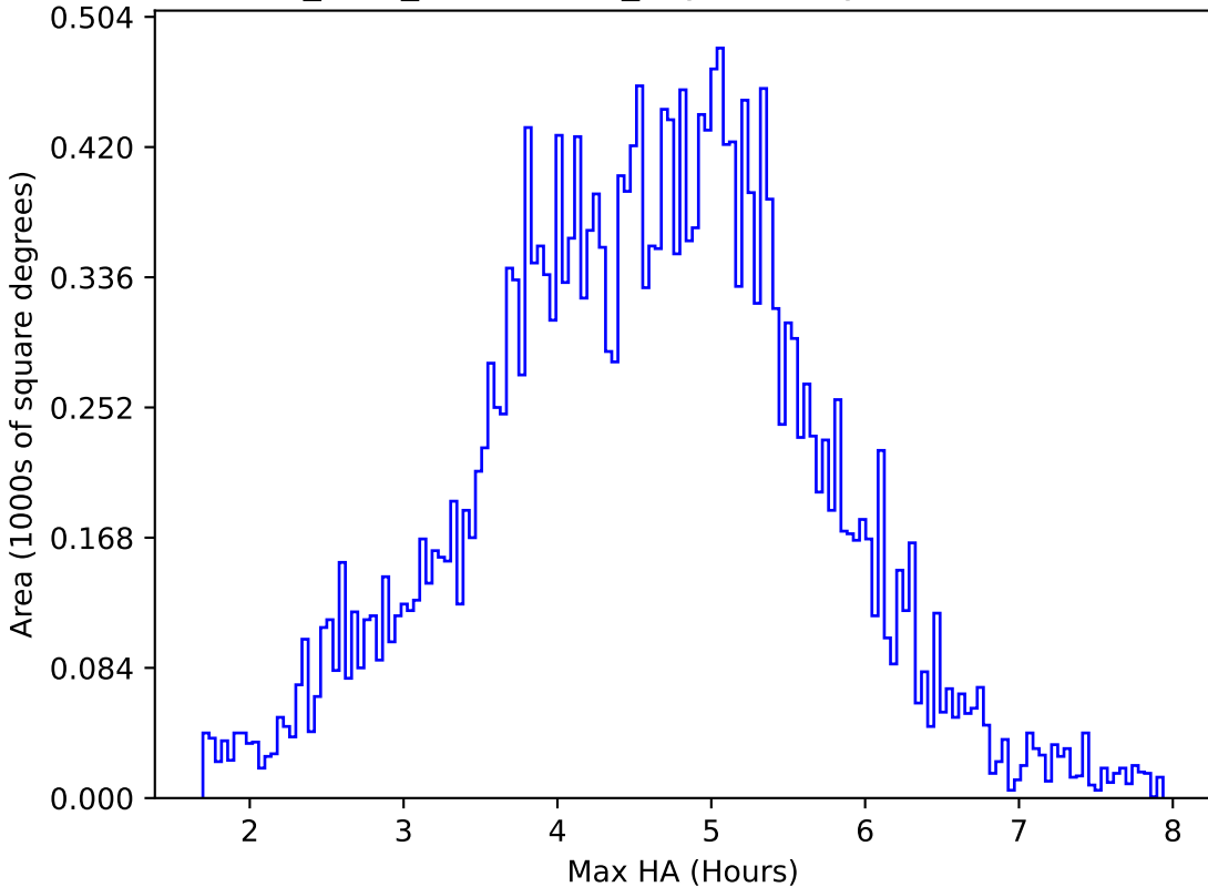
start_date_do-360v3.4_10yrs All sky i band: Max HA
