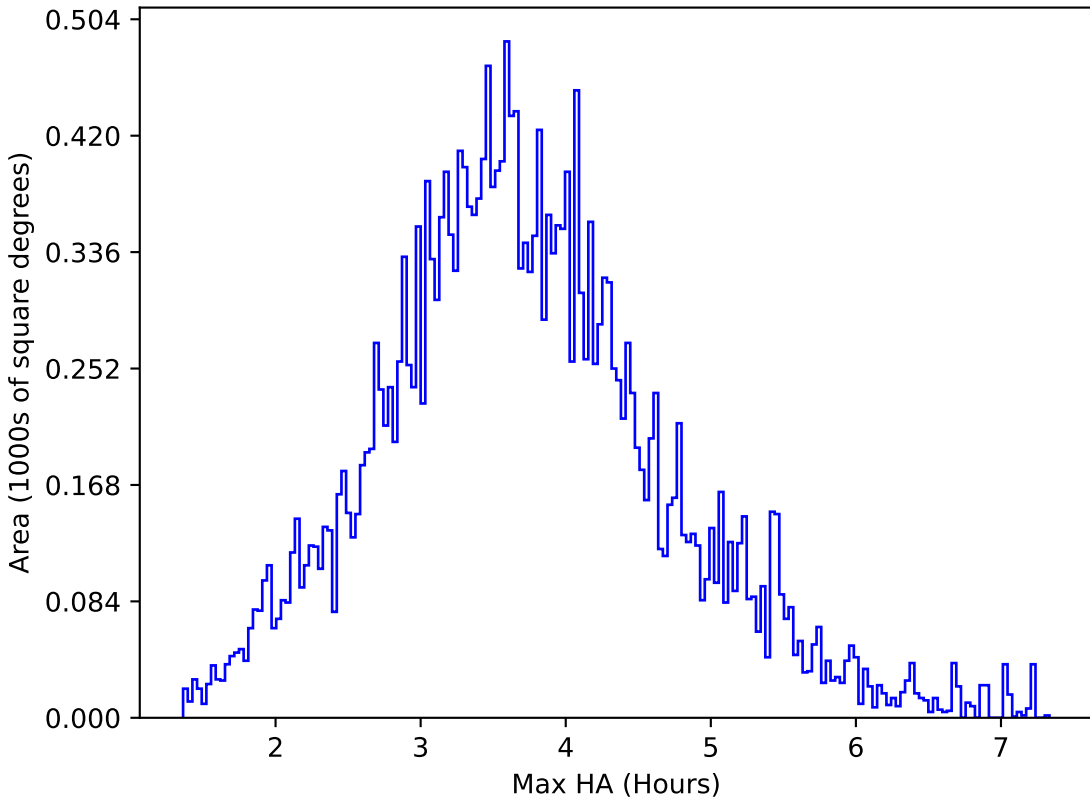
start_date_do-360v3.4_10yrs All sky g band: Max HA
