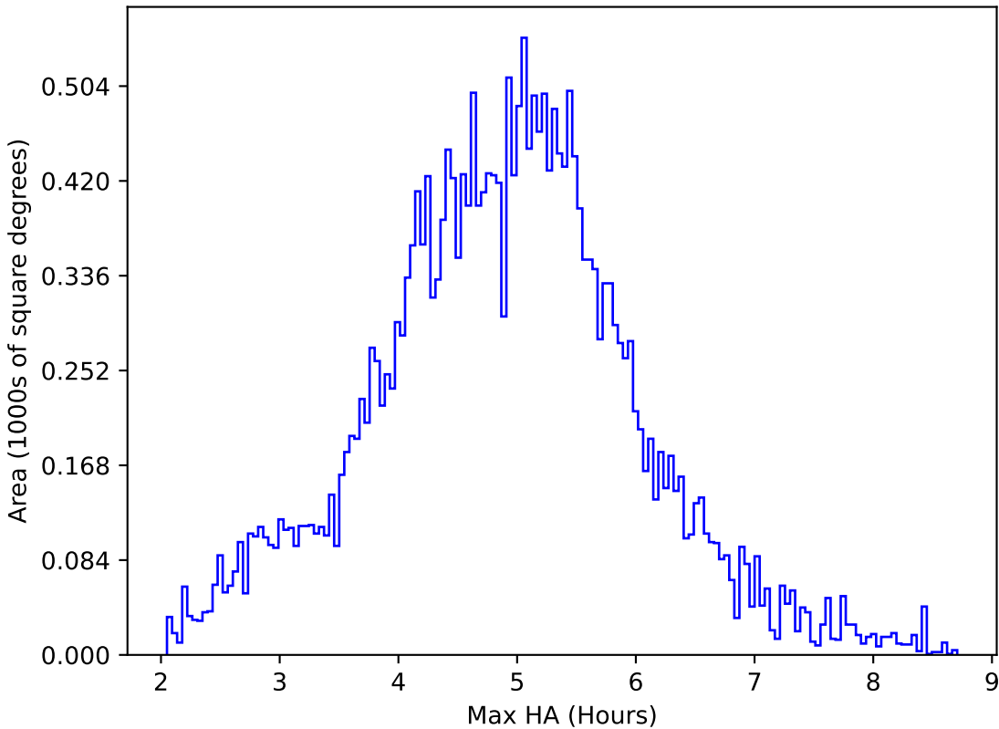
start_date_do-360v3.4_10yrs All sky all bands: Max HA
