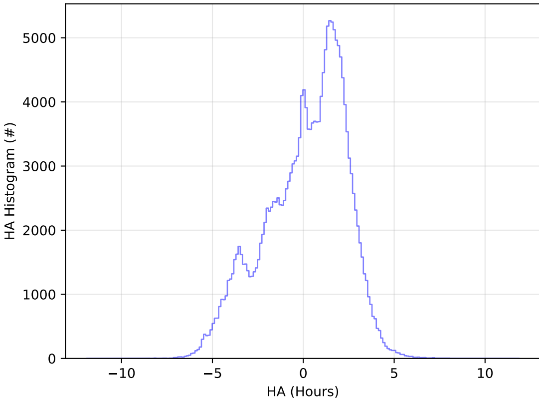
start_date_do-360v3.4_10yrs WFD g band: HA Histogram
