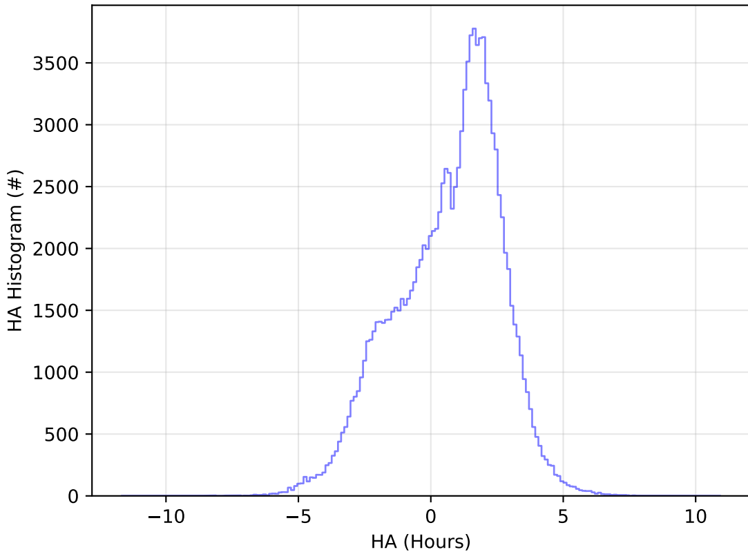
start_date_do-360v3.4_10yrs All sky u band: HA Histogram
