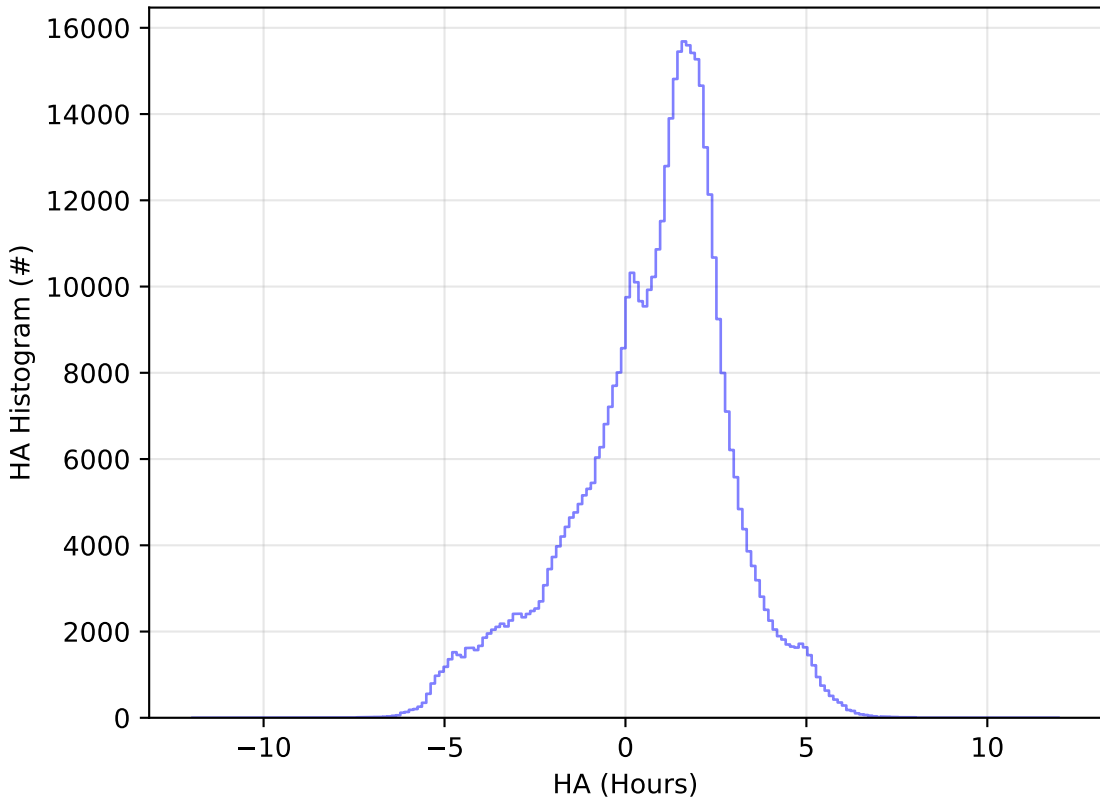
start_date_do-360v3.4_10yrs All sky i band: HA Histogram
