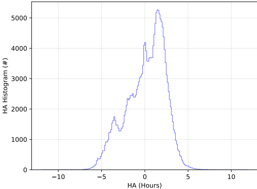
start_date_do-360v3.4_10yrs All sky g band: HA Histogram
