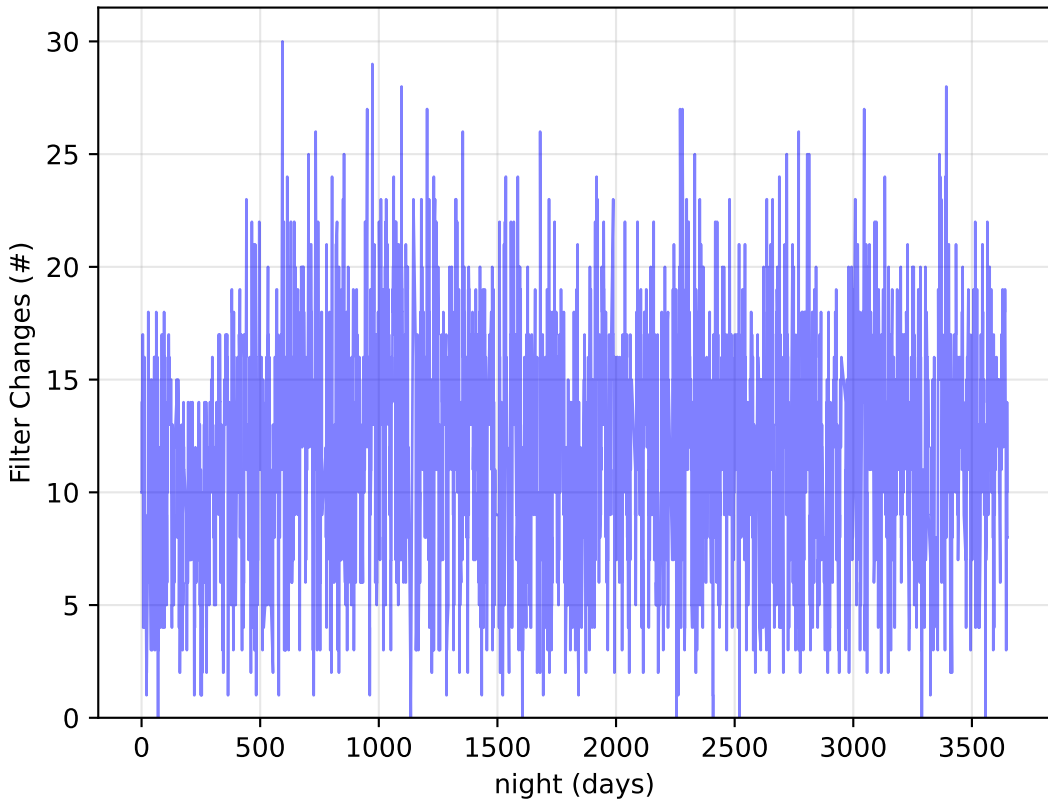
start_date_do-360v3.4_10yrs Per Night: Filter Changes
