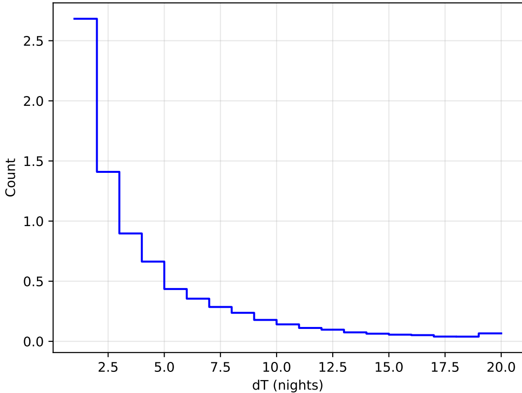
start_date_do-360v3.4_10yrs WFD all bands: DeltaNight Histogram 1e6
